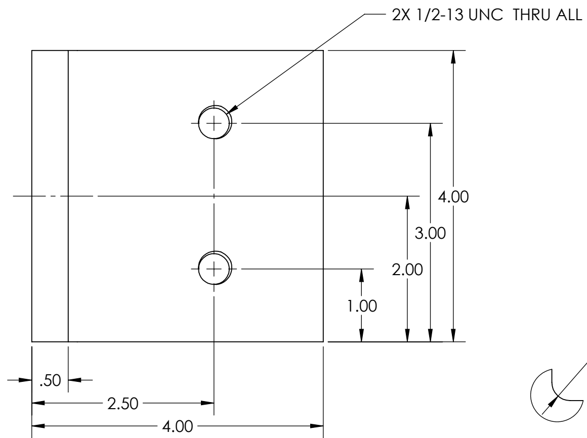
DETAIL B
